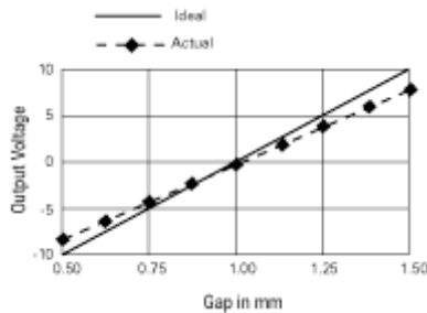
Figure 10 Sensitivity Error – The slope of the actual measurements deviates from the ideal slope.
