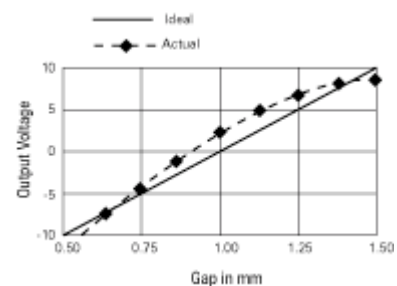
Figure 12 Linearity Error – Measurement data is not on a straight line.
