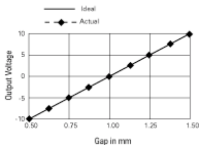
Figure 9 Sensitivity – The slope of the line is the sensitivity; in this case 1V/0.05mm.
