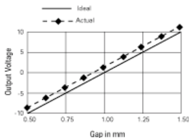
Figure 11 Offset Error – A constant value is added to all measurements.
