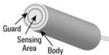
Figure 4 Capacitive sensor probe components
