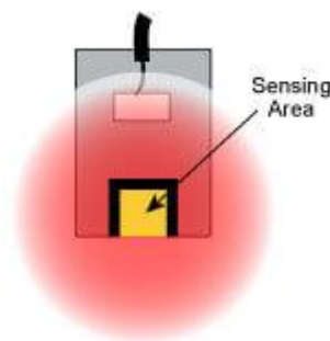
Figure 5 Cutaway view showing an unguarded sensing area electric field
