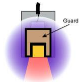
Figure 6 Cutaway showing the guard field shaping the sensing area electric field
